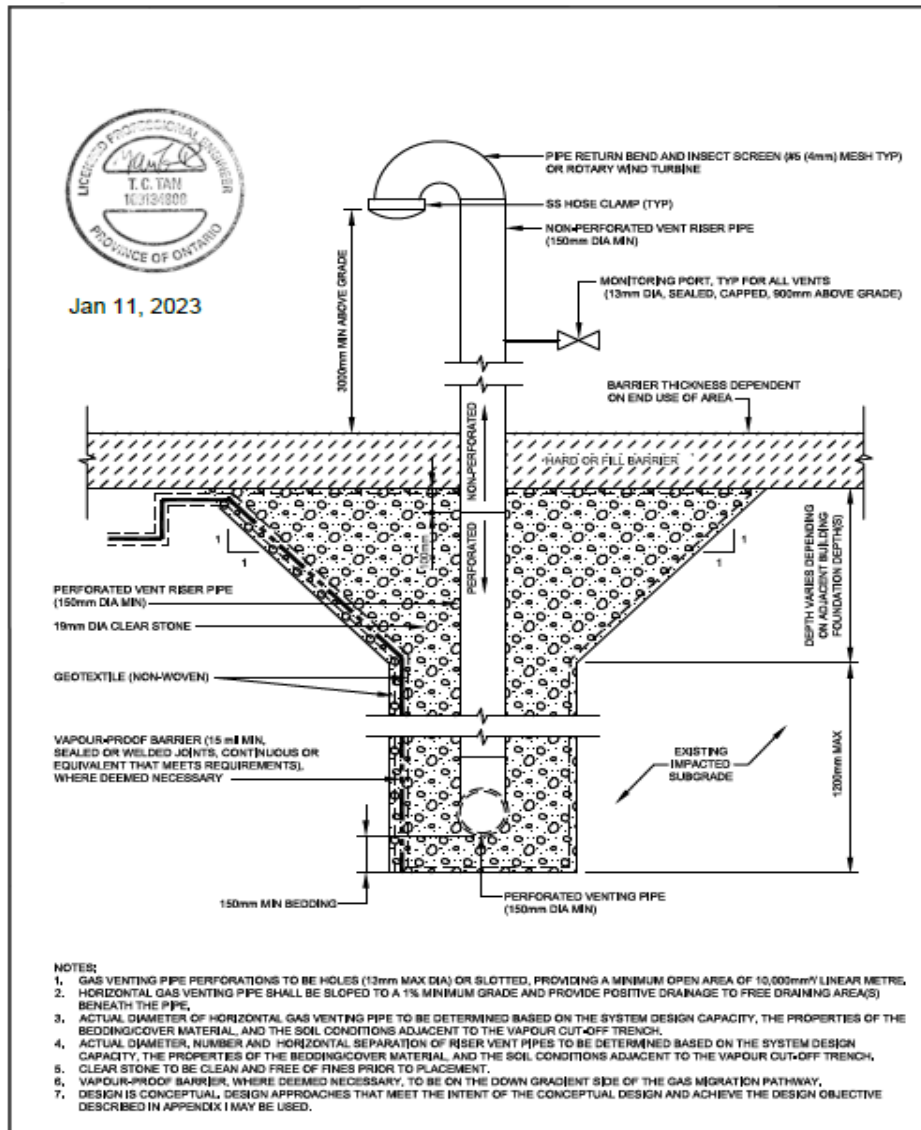
FIGURE I-9 Conceptual Design of Vapour Cut-off Trench Passive Relief, Collection, and Venting System
