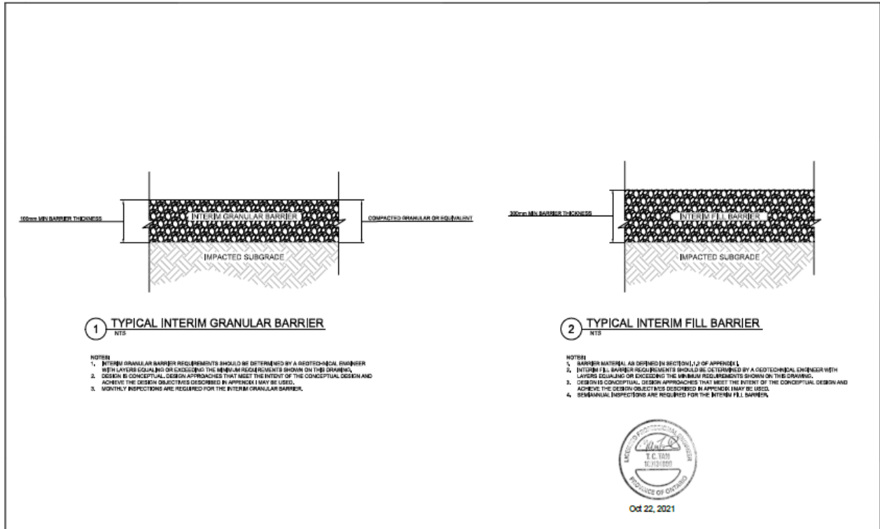
FIGURE I-3 Conceptual Design of Interin Cap Barrier
