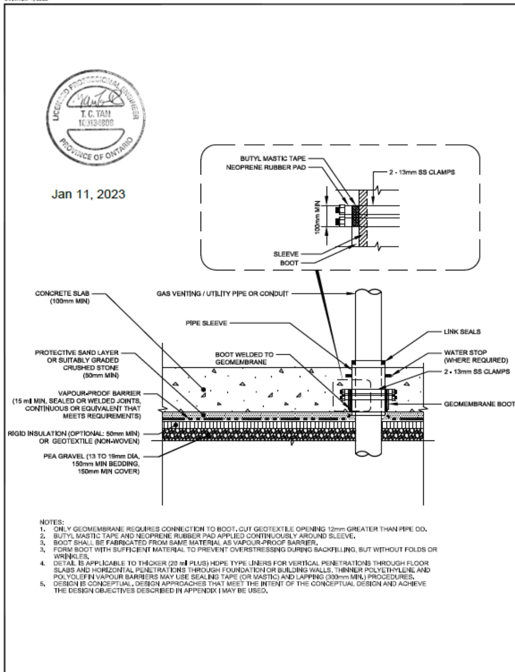
FIGURE I-10 Conceptual Design for Conduit and Pipe Penetrations Passive Relief, Collection, and Venting System
