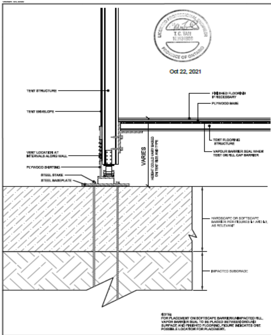
FIGURE 1-11 Conceptual Design of Vapor Mitigation System for Temporary Tent Structures
