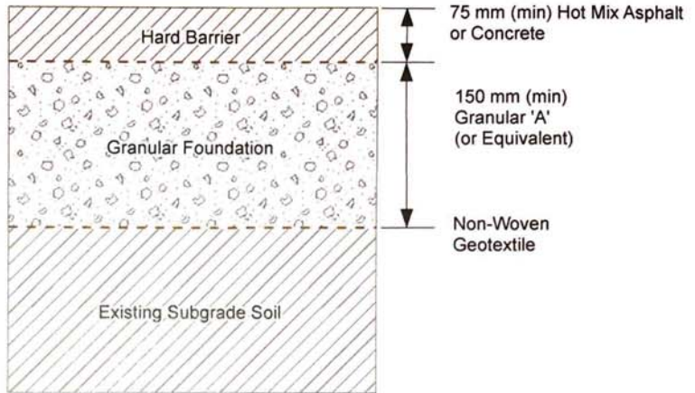
Typical Hard Cap Barrier
