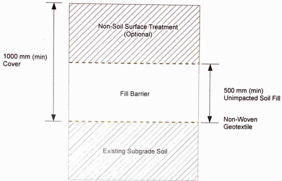
Typical Fill Cap Barrier
