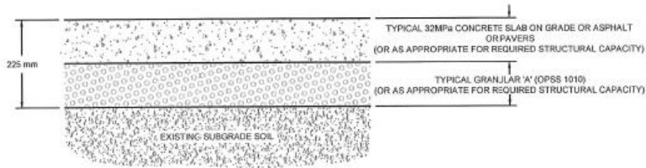
TYPICAL HARD CAP (ASPHALT, CONCRETE) DETAIL
