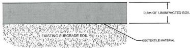
TYPICAL SHALLOW SOIL CAP DETAIL
